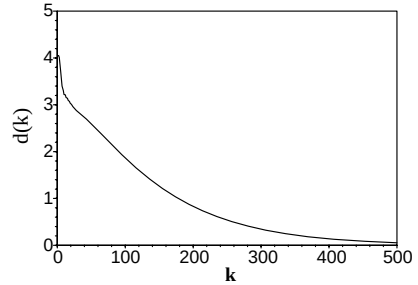
FIGURE 3.4. Convergence of algorithm (3.6)–(3.8) with \alpha = 300
