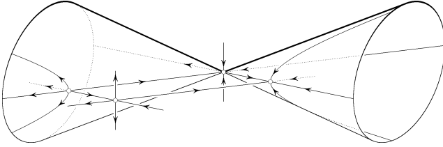
FIGURE 1.3. Riccati flow on \overline{S(1, 2)} .
