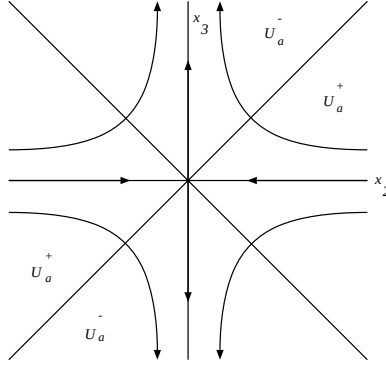
FIGURE 3.1. Flow around a saddle point
